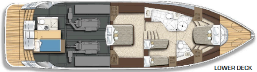
LOWER DECK
